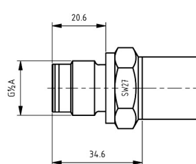
Fig. 9 - G 1/2 M, frontal diaphragm
